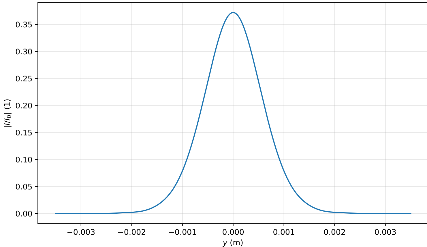
Intensity profile I(x=0, y, z=3.662)/I_0 , P_{in}=0.4P_{cr} , artificial time
